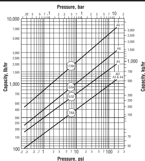
Model A & AI Series Capacity—175 psi
