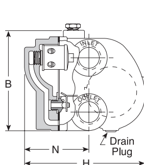
Model A Traps
