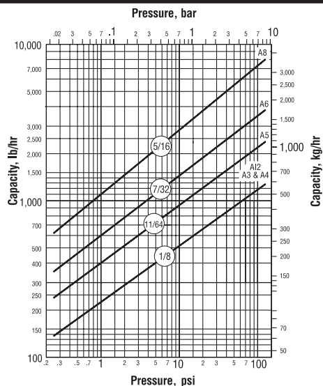
Model A & AI Series Capacity—125 psi
